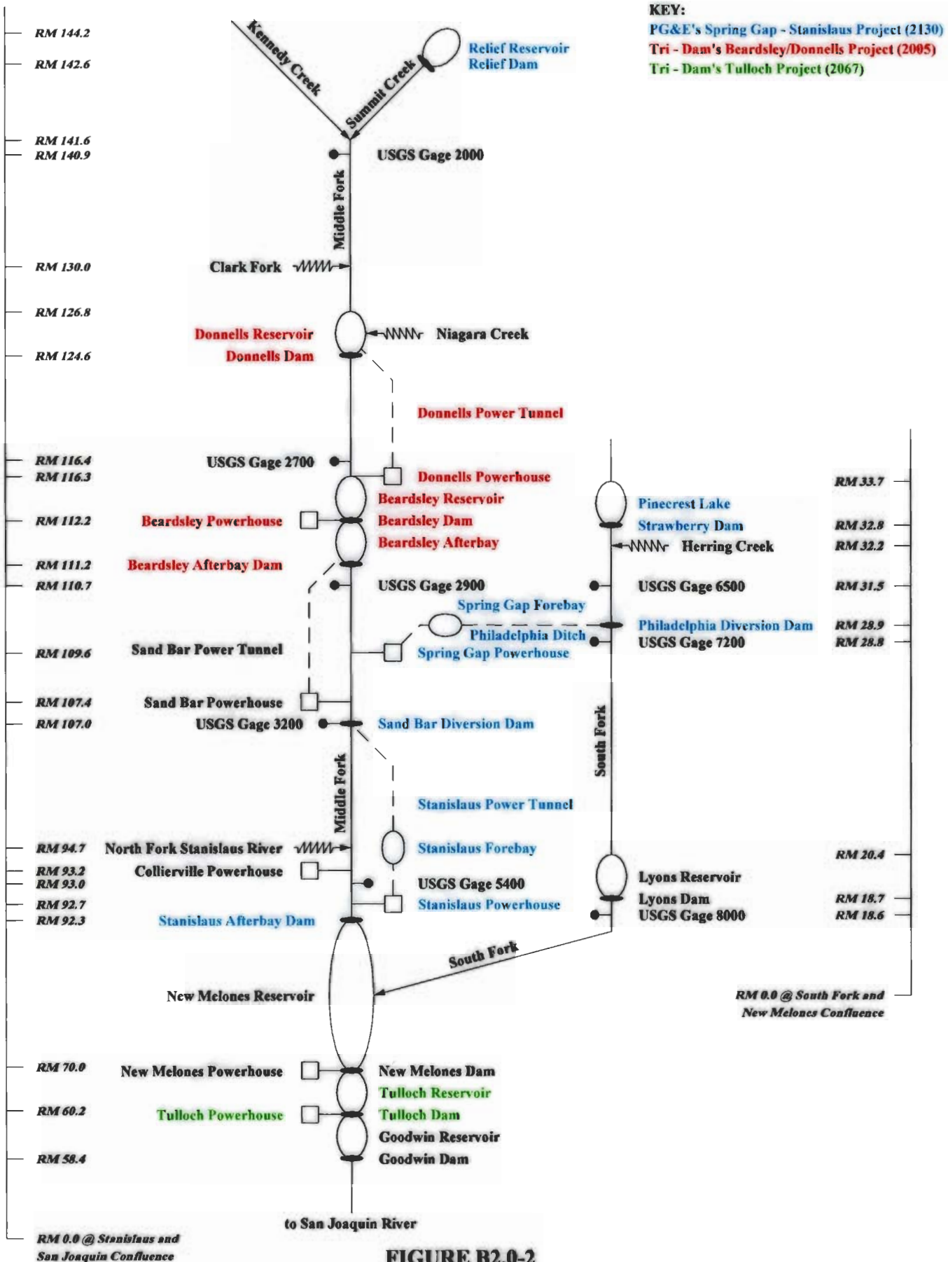
Schematic Diagram of Major Physical Characteristics of the Middle Fork and South Fork of the Stanislaus River.
